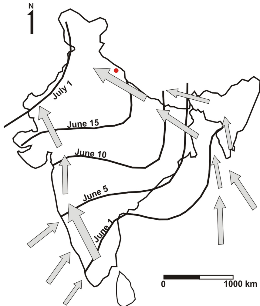
Fig. 1. Map of India showing mean annual arrival date of the Indian Summer Monsoon (lines with dates) and the principal trajectories of moisture masses associated with monsoon (arrows). The red circle indicates the location of Chulerasim cave. (For interpretation of the references to colour in this figure legend, the reader is referred to the web version of this article.)
