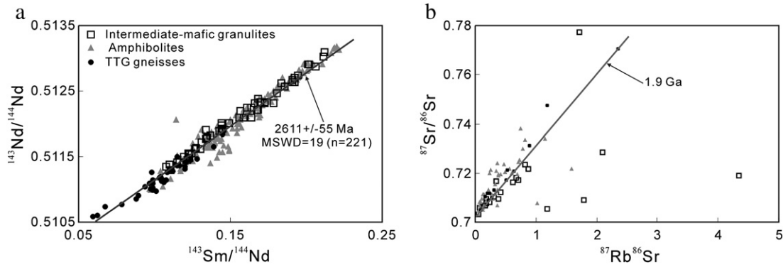
Fig. 2. Sm–Nd isotopic data (a) and Rb–Sr isotopic data (b) for rocks from the granulite terrains.
